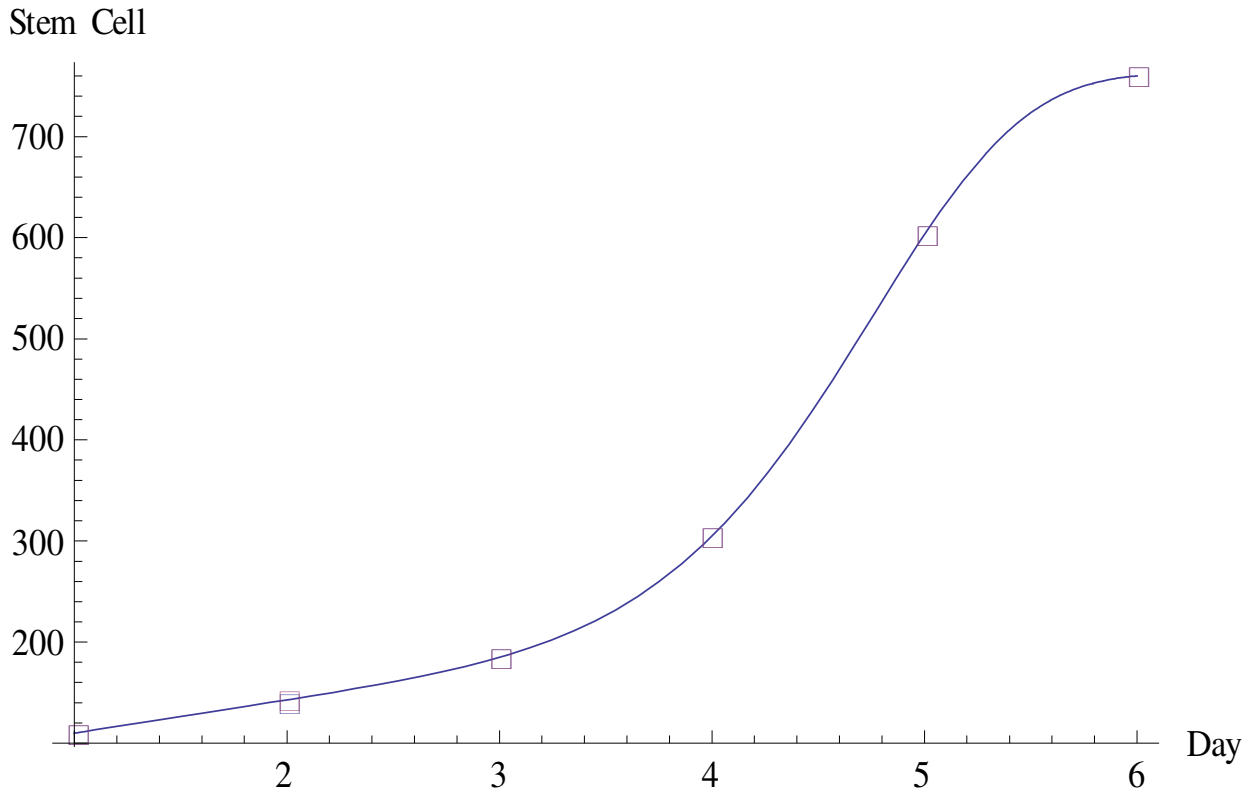
Figure 2. Scatter Plot of Observed and Estimated Number of Embryonic Stem Cells Using Hyperbolic H3 Model square represents observed number of embryonic stem cells circle represents estimated number of embryonic stem cells using H3
