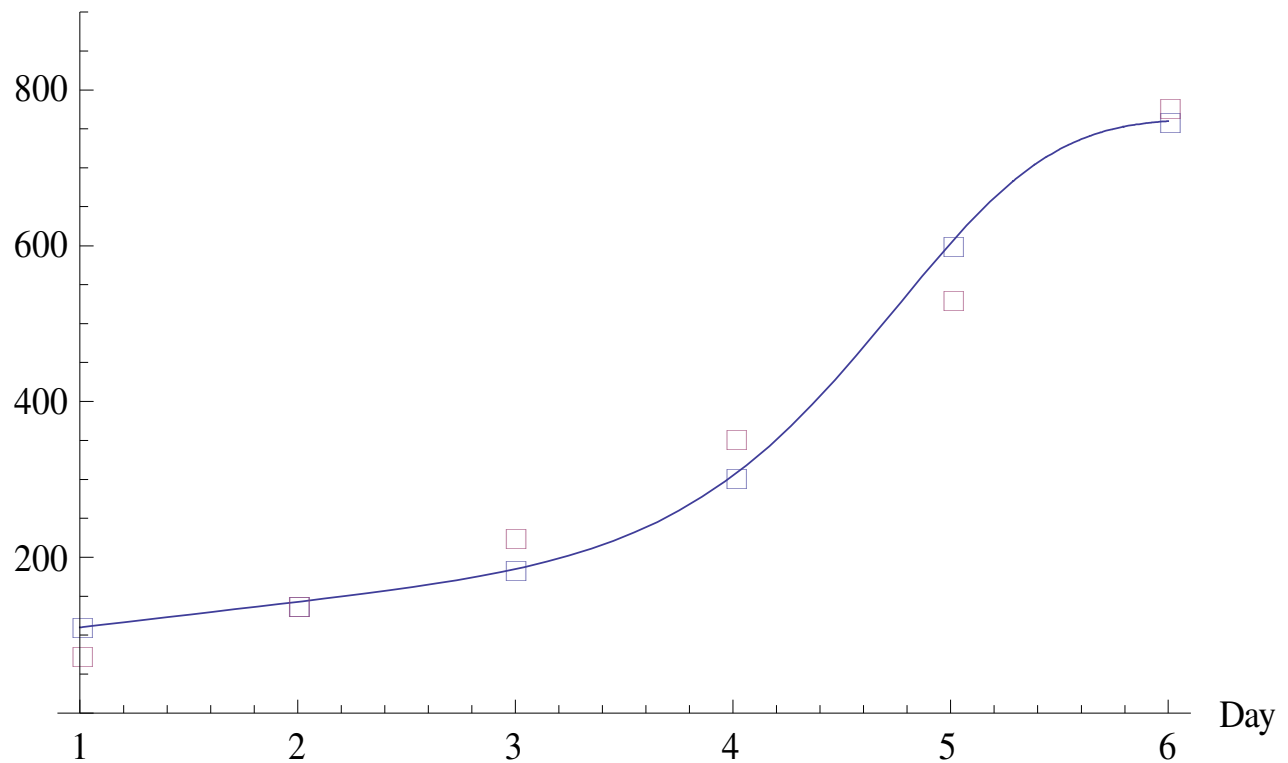
Figure 3. Scatter Plot of Observed and Estimated Number of Embryonic Stem Cells Using the Deasy Model
