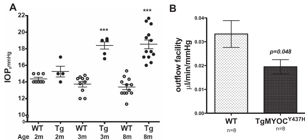
FIGURE 1. (A) Intraocular pressure elevation in 2-, 3-, and 8-month-old WT and Tg-MYOC Y437H littermates (two-tailed Student's t -test; *** P < 0.0001; versus WT littermates; n = 4–8 eyes at 2 months; n = 8–12 eyes for 3 and 8 months). (B) Reduced outflow facility in 10-month-old Tg-MYOC Y437H mice (two-tailed Student's t -test; P = 0.048; n = 8 eyes).
