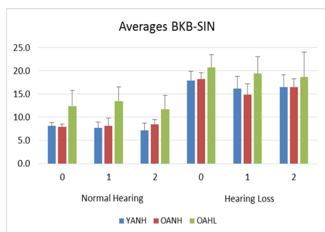
Figure 2: Older adults with hearing loss have significantly higher average BKB-SIN scores, with a higher score indicating worse performance, compared to young adults and older adults with normal hearing during Level 0, 1, and 2 surface translations. All adults perform significantly worse under the hearing loss condition. YANH=Young Adults with Normal Hearing; OANH=Older Adults with Normal Hearing; O AHL=Older Adults with Hearing Loss. Normal Hearing=Normal Hearing/Hearing Aid condition; Hearing Loss=Simulated Hearing Loss/No Hearing Aid condition.
